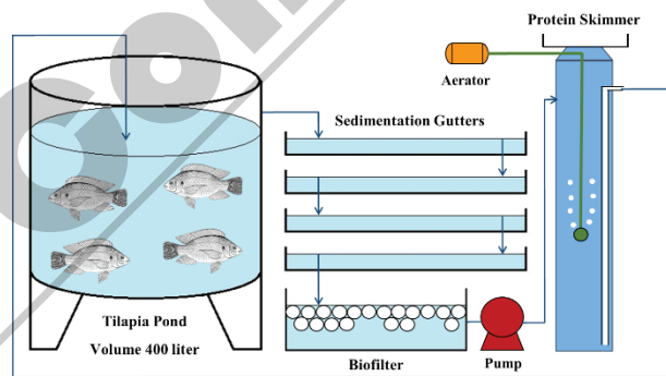
Figure 1 Diagram of tilapia pond in water recirculation systems
